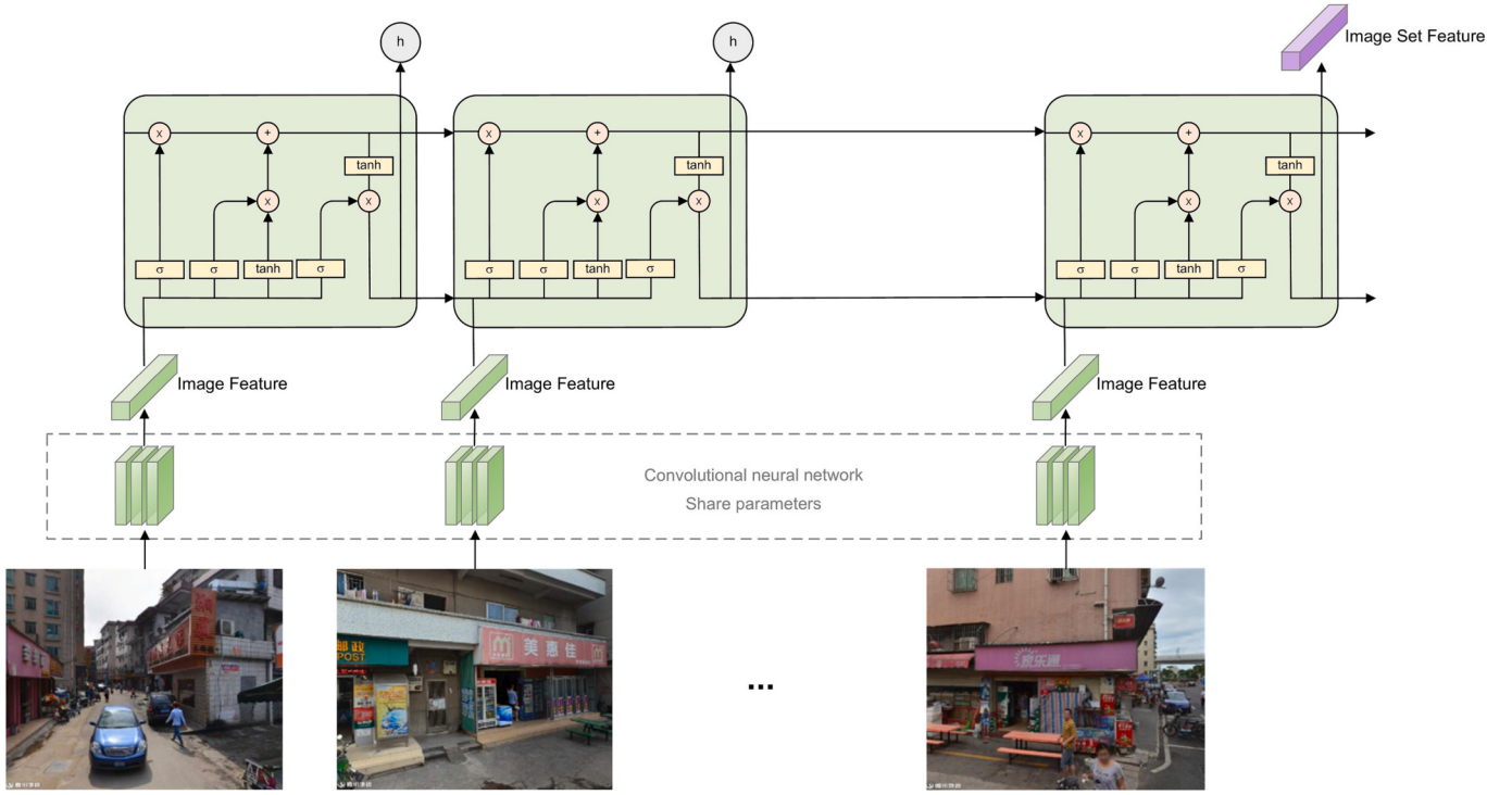
Fig. 3. Structure of the Vision-LSTM.
