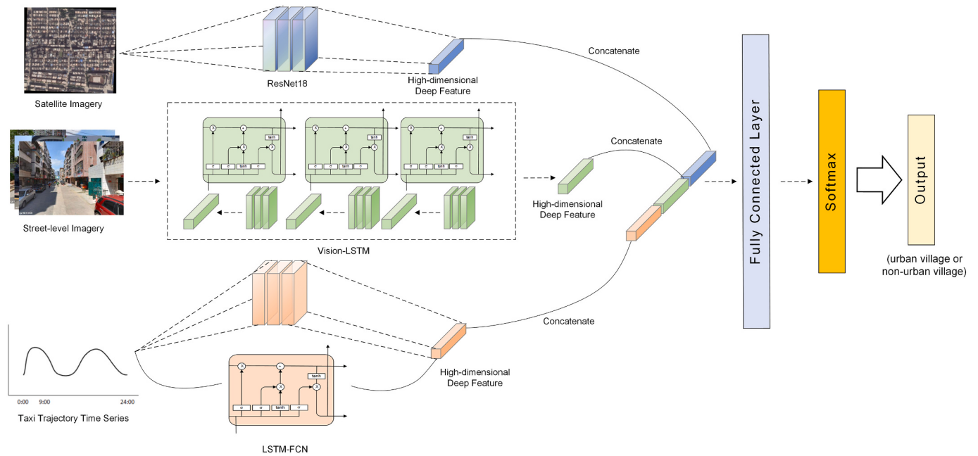
Fig. 5. Structure of multimodal model.
