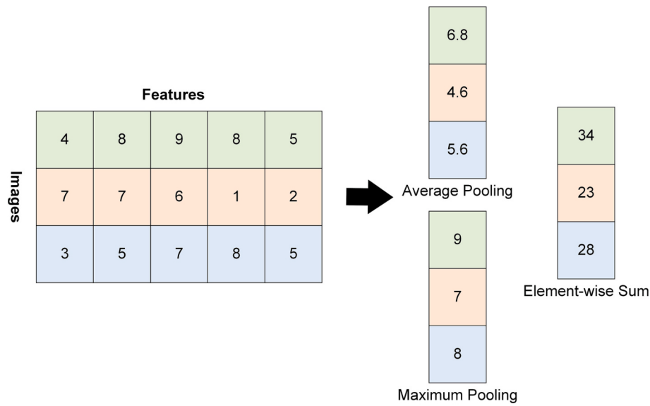
Fig. 2. Average pooling, maximum pooling and element-wise sum for the fusion of street-level image features, in comparison of our proposed Vision-LSTM (Fig. 3).
